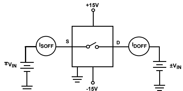
FIGURE 3. OFF LEAKAGE CURRENT TEST CIRCUIT
