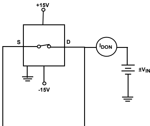
FIGURE 4. “ON” LEAKAGE CURRENT TEST CIRCUIT
