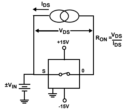
FIGURE 2. "ON" RESISTANCE TEST CIRCUIT
