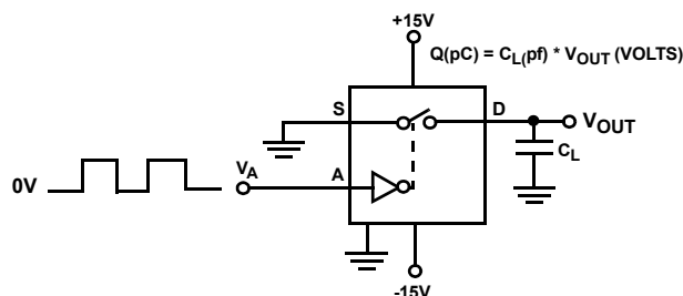
FIGURE 6. CHARGE INJECTION TEST CIRCUIT
