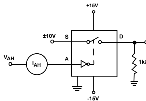
FIGURE 11. INPUT LEAKAGE CURRENT TEST CIRCUITS
