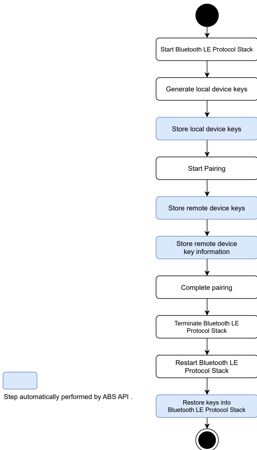
Figure 9-2 Bonding procedure
