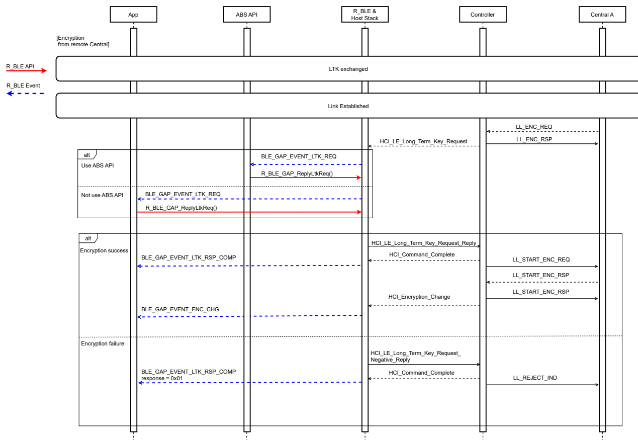
Figure 9-8 Sequence of response to an encryption request from remote device(Central)
