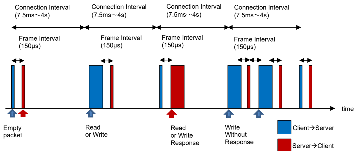
Figure 1-6 Read and Write
