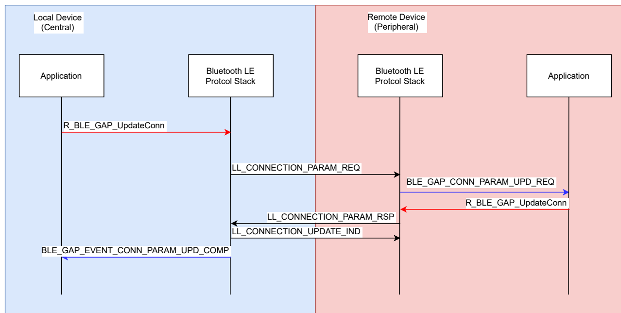
Figure 8-5 Sequence chart when updating connection parameters
