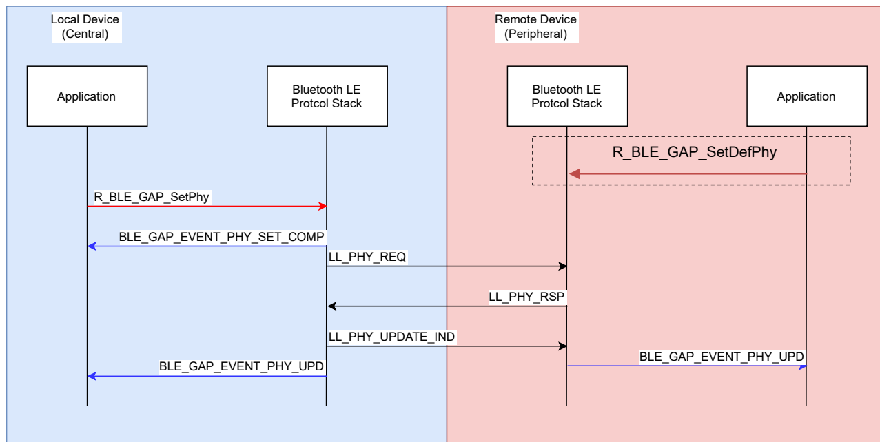
Figure 8-1 Sequence chart when changing PHY
