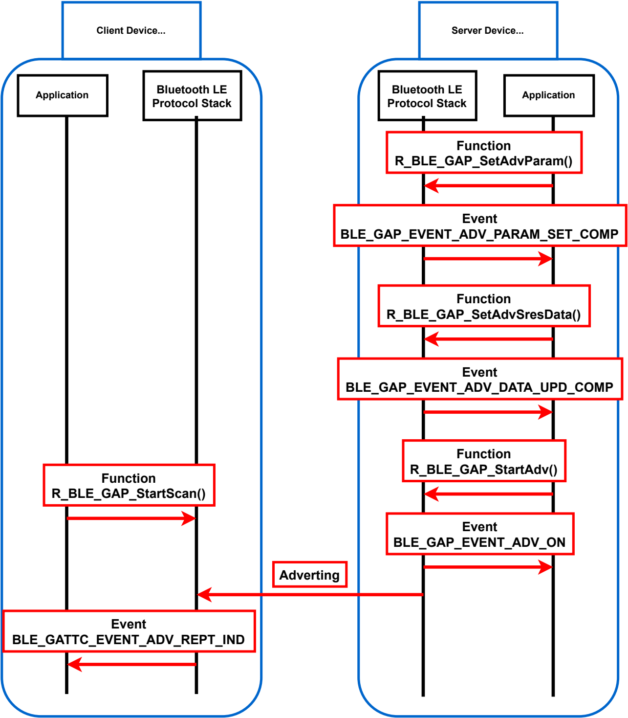
Figure 10-8 Flow of Broadcast operation
