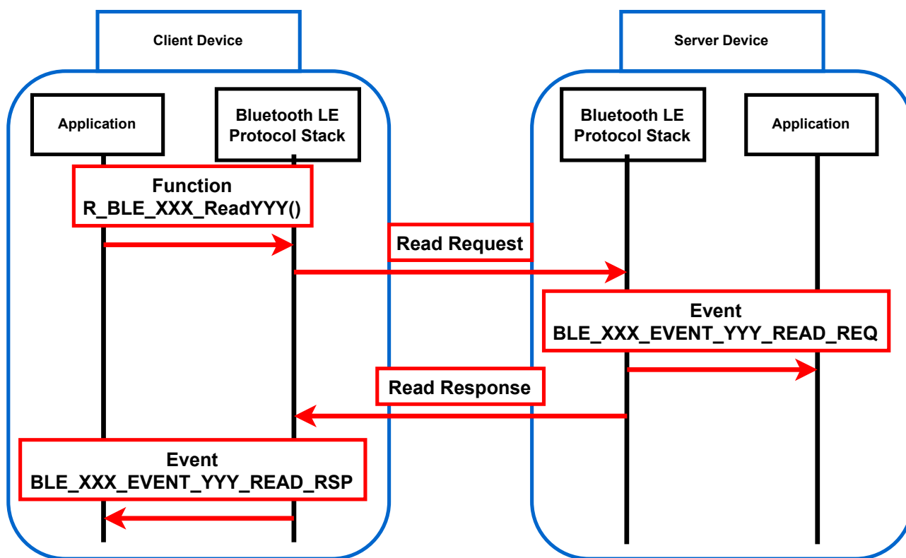
Figure 10-2 Flow of Read operation
