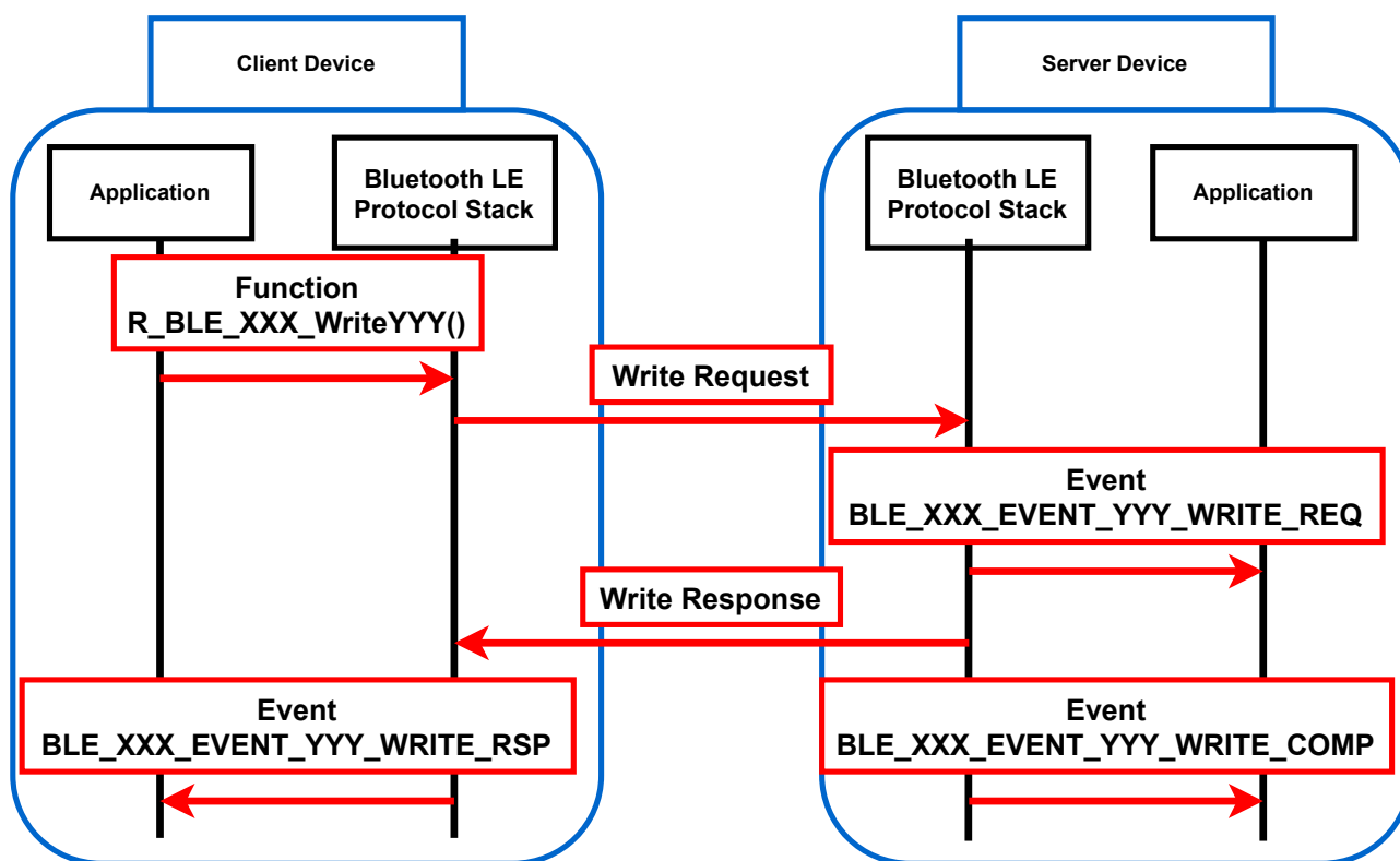
Figure 10-3 Flow of Write operation
