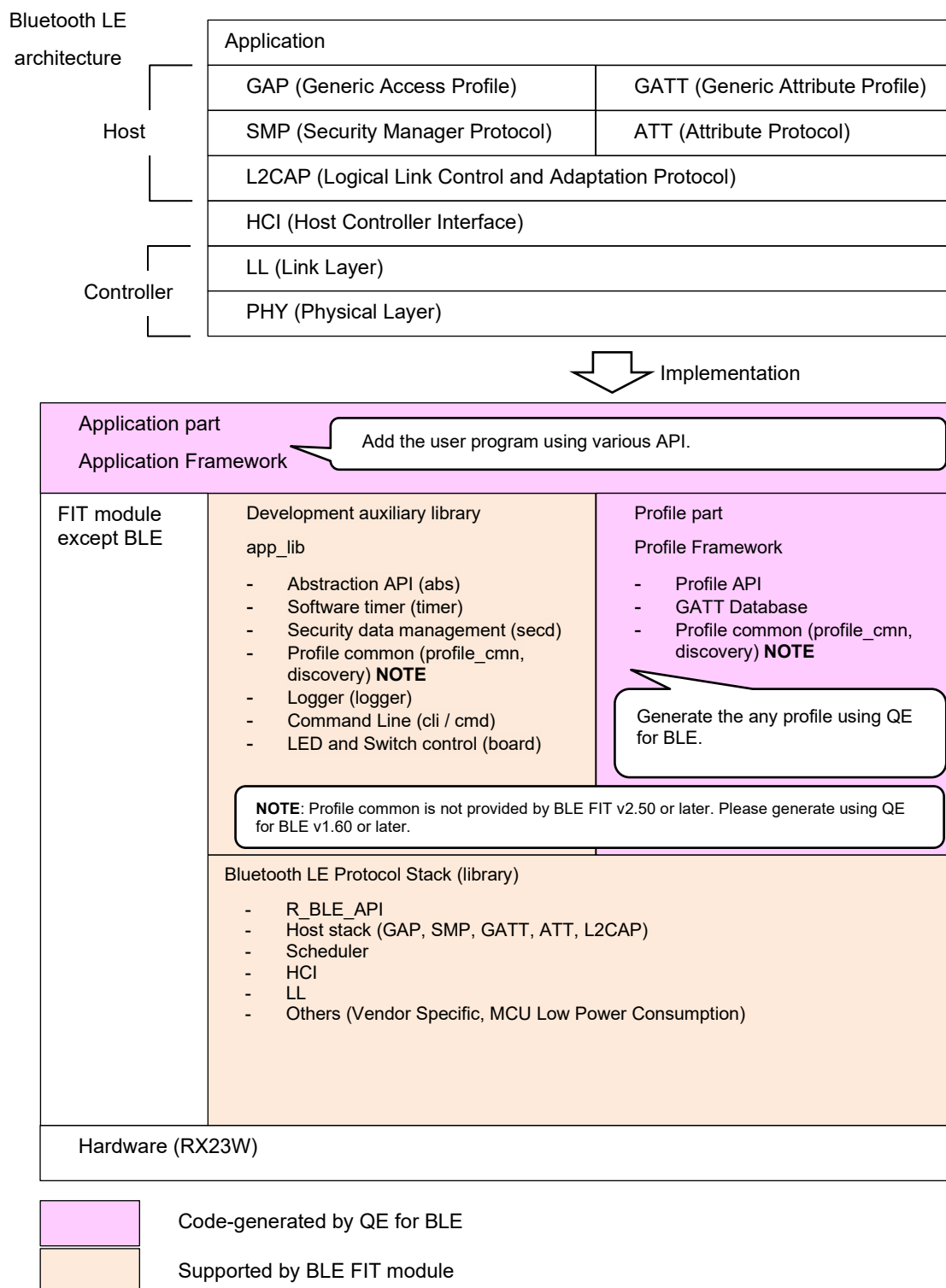
Figure 1-10 Software structure
