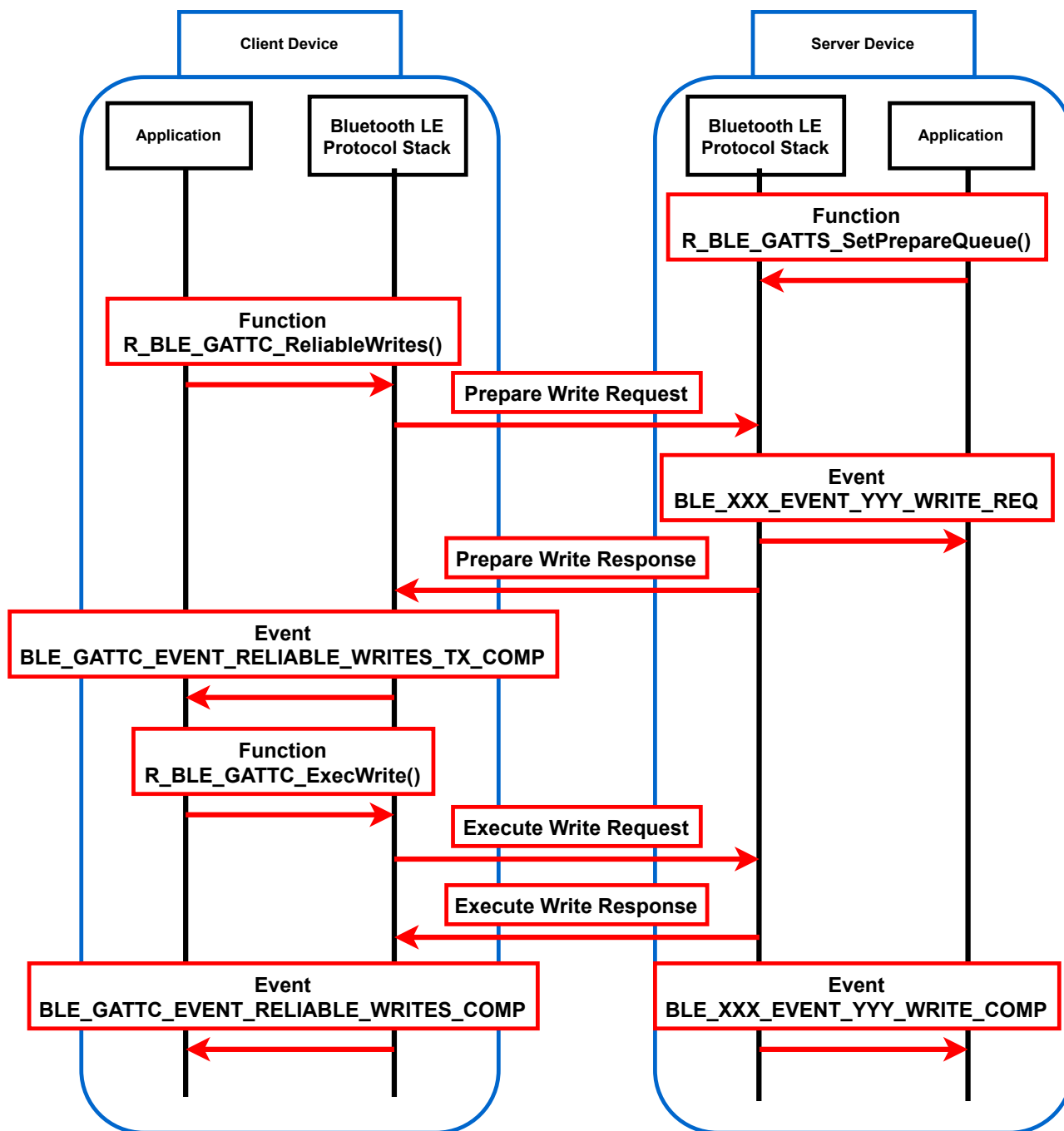
Figure 10-7 Flow of ReliableWrites operation
