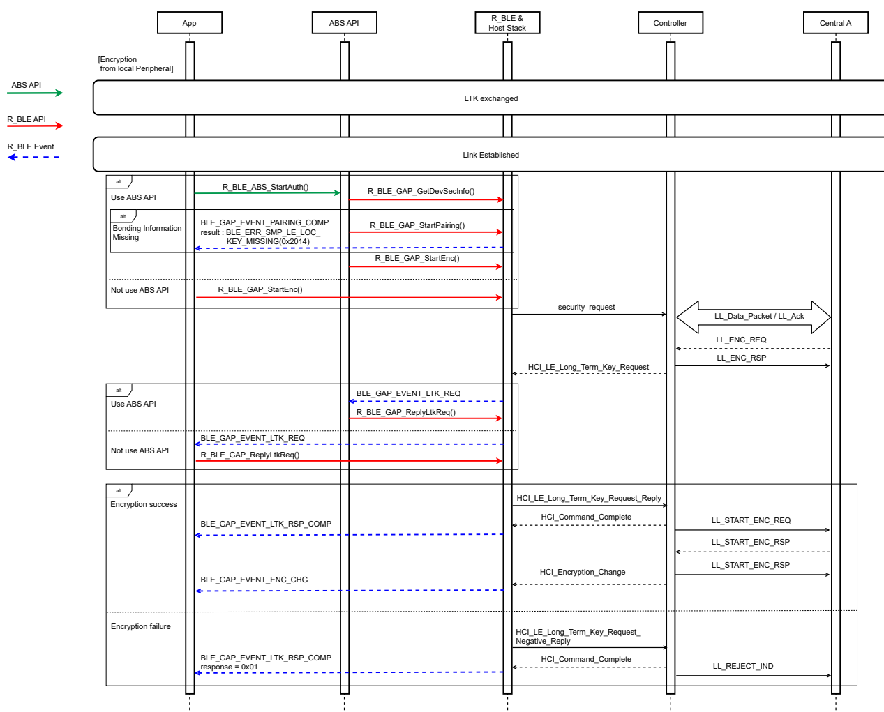
Figure 9-7 Sequence of encryption request from local device(Peripheral)
