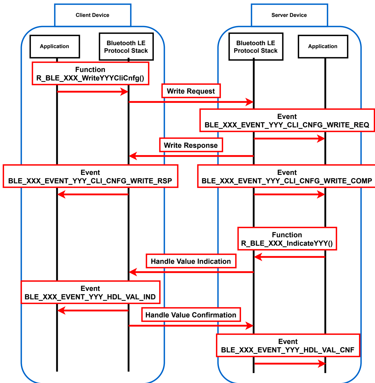
Figure 10-6 Flow of Indication operation
