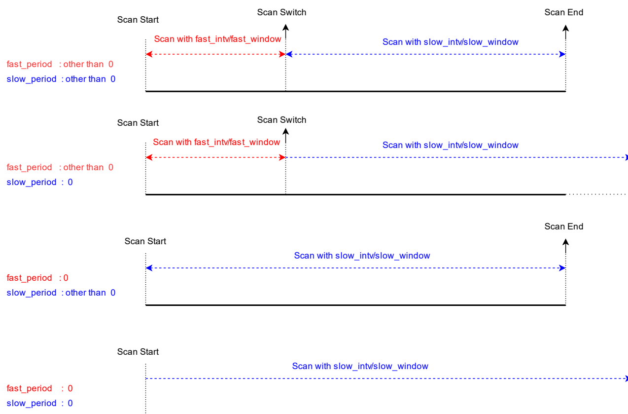
Figure 6-2 The relationship between the fast scan and slow scan
