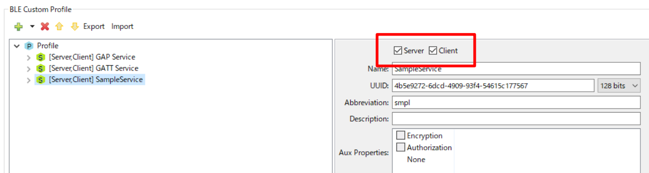
Figure 7-7 Select GATT Role on Service Screen
