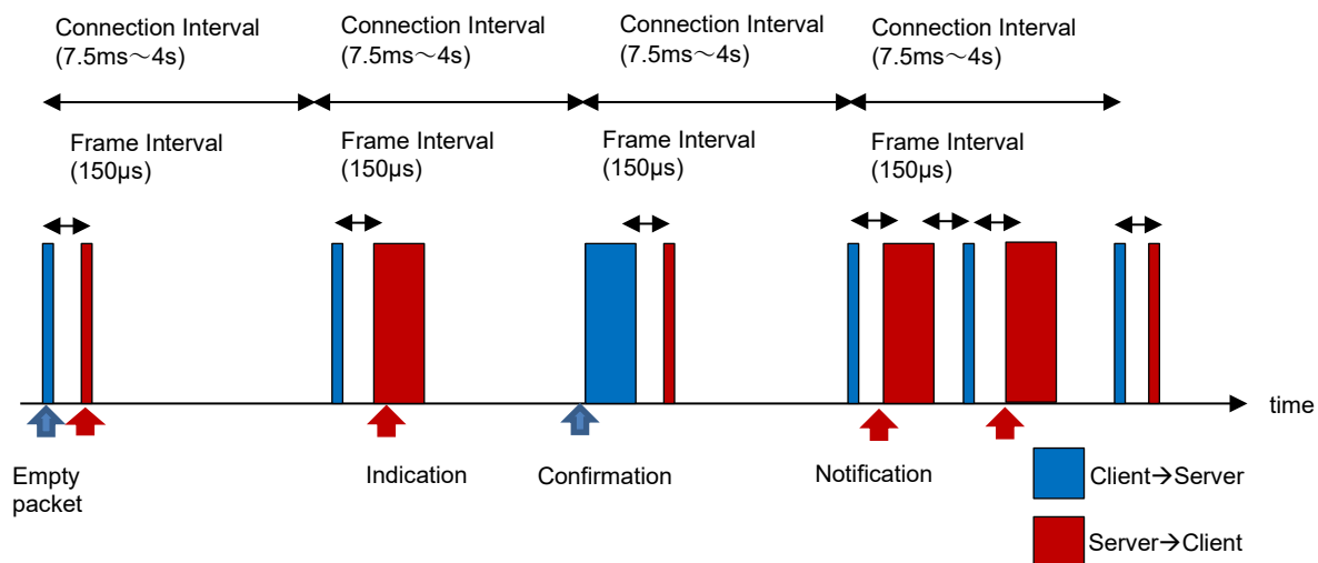
Figure 1-7 Indication and Notification
