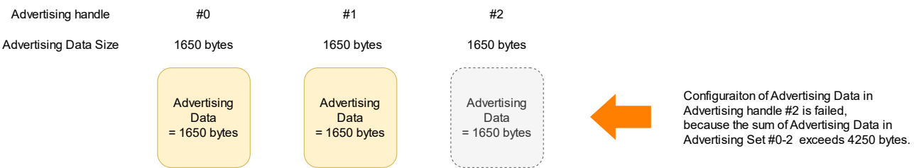
Figure 5-8 Failed sample of setting Advertising Data
