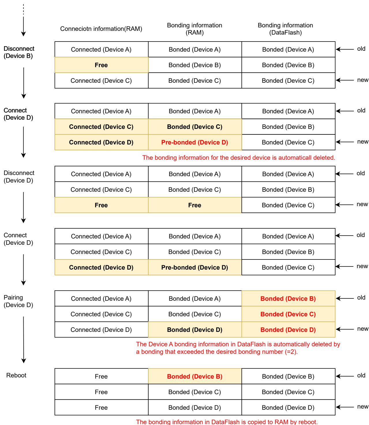
Figure 9-4 Bonding information management in RAM, DataFlash (2)
