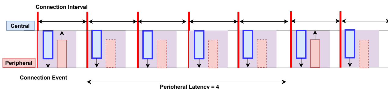
Figure 8-3 Schematic diagram of Peripheral Latency and connection event
