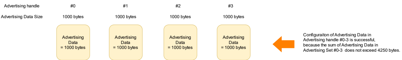
Figure 5-7 Successful sample of setting Advertising Data
