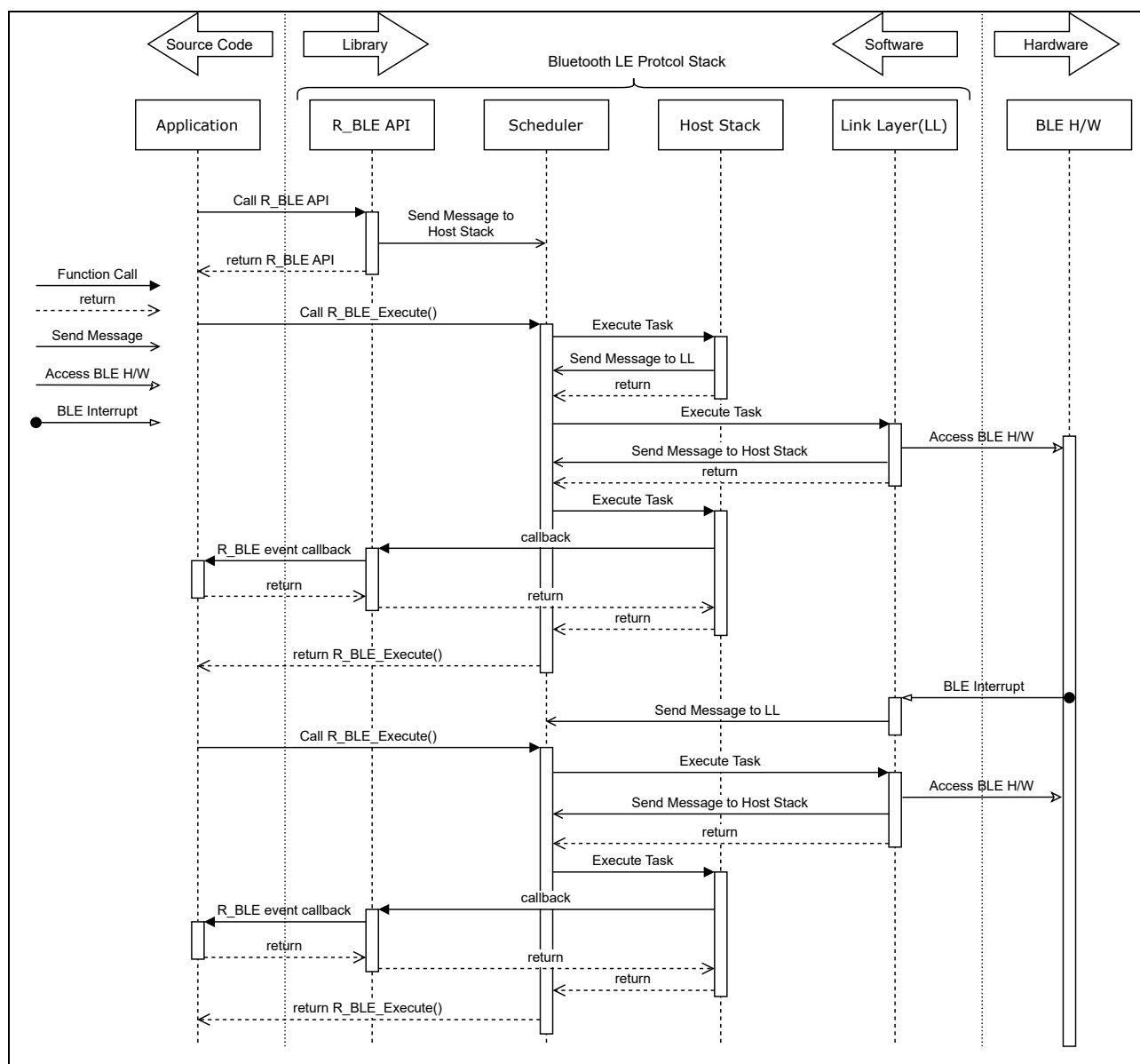
Figure 3-2 Basic sequence chart of Bluetooth LE Protocol Stack
