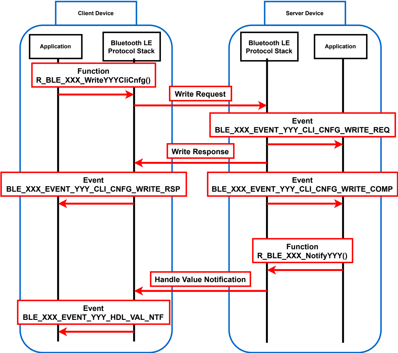
Figure 10-5 Flow of Notification operation
