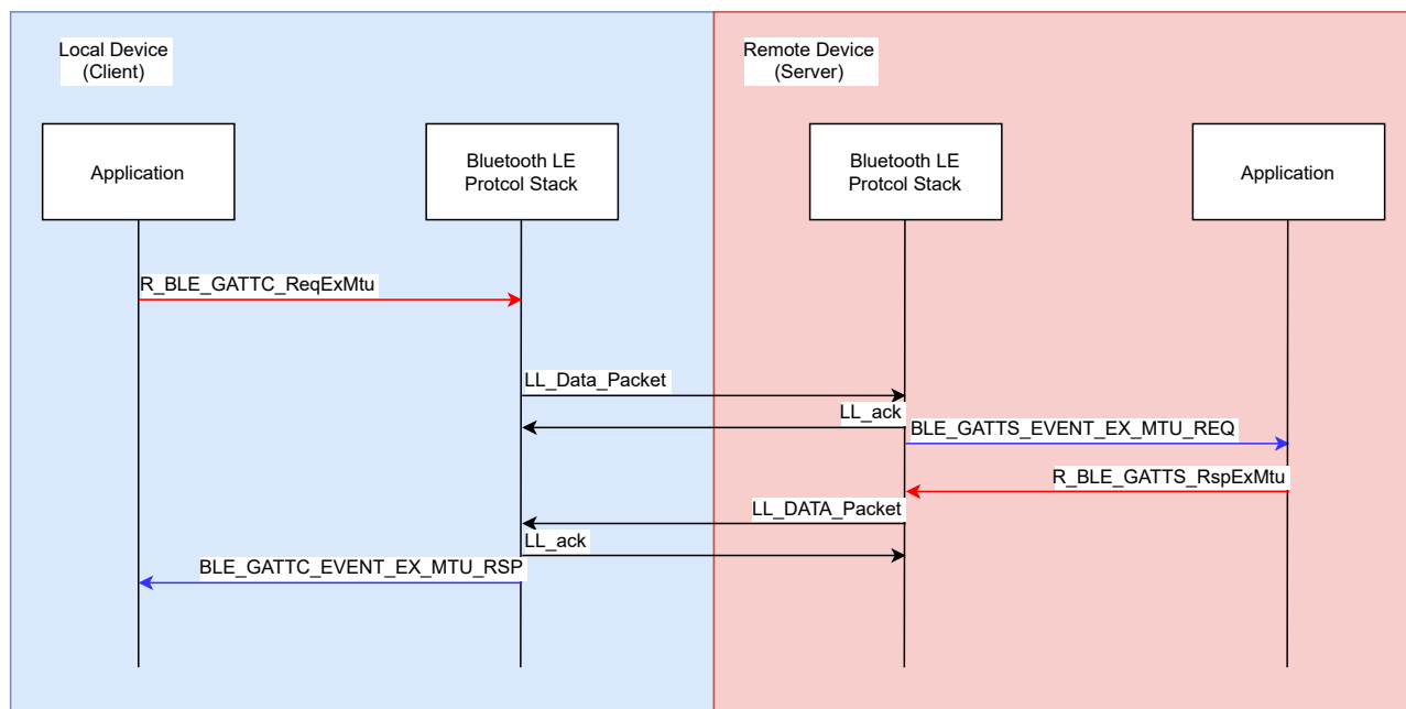
Figure 8-6 Sequence chart when changing MTU
