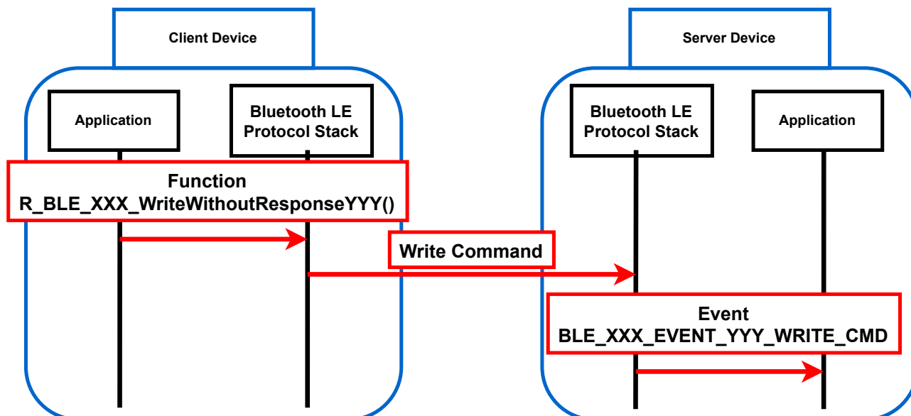
Figure 10-4 Flow of WriteWithoutResponse operation
