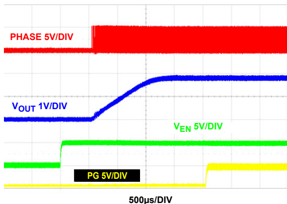
FIGURE 18. START-UP AT 4A LOAD (PWM)
