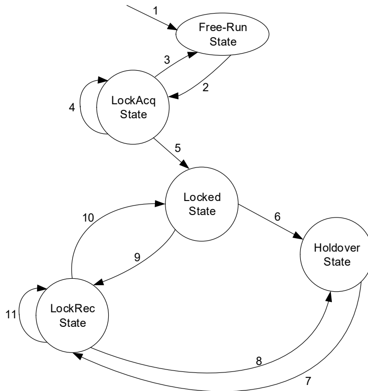
Figure 11. DPLL Automatic State Machine
