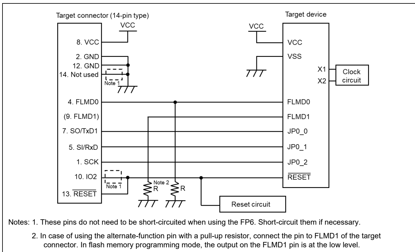
Figure 3.20 Example of a Circuit for V850E2 (CSI)
