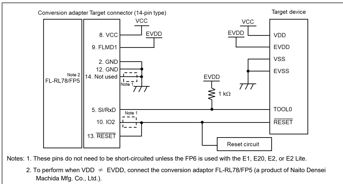
Figure 3.4 Example of a Circuit for RL78 Family ( VDD \neq EVDD )
