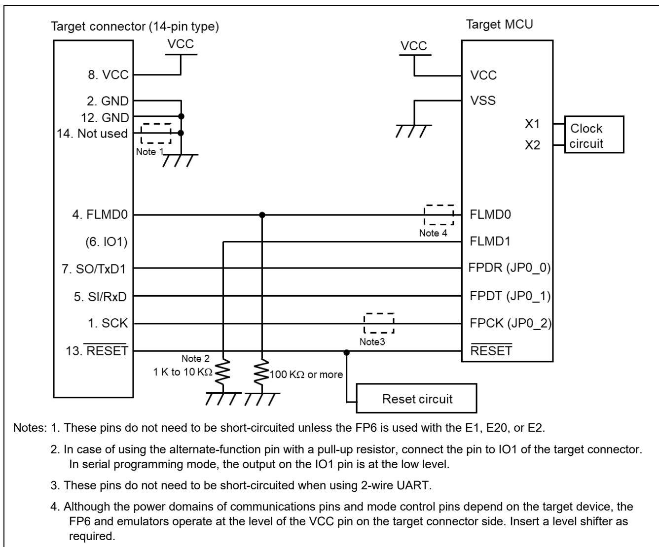
Figure 3.9 Example of a Circuit for RH850 Family (2-wire UART or CSI) (Case of RH850/F1x)
