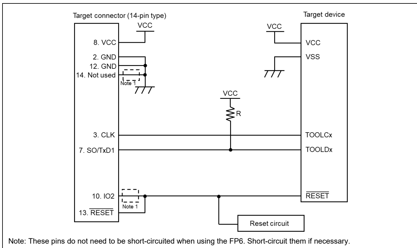
Figure 3.18 Example of a Circuit for 78K0 (TOOLCx and TOOLDx)
