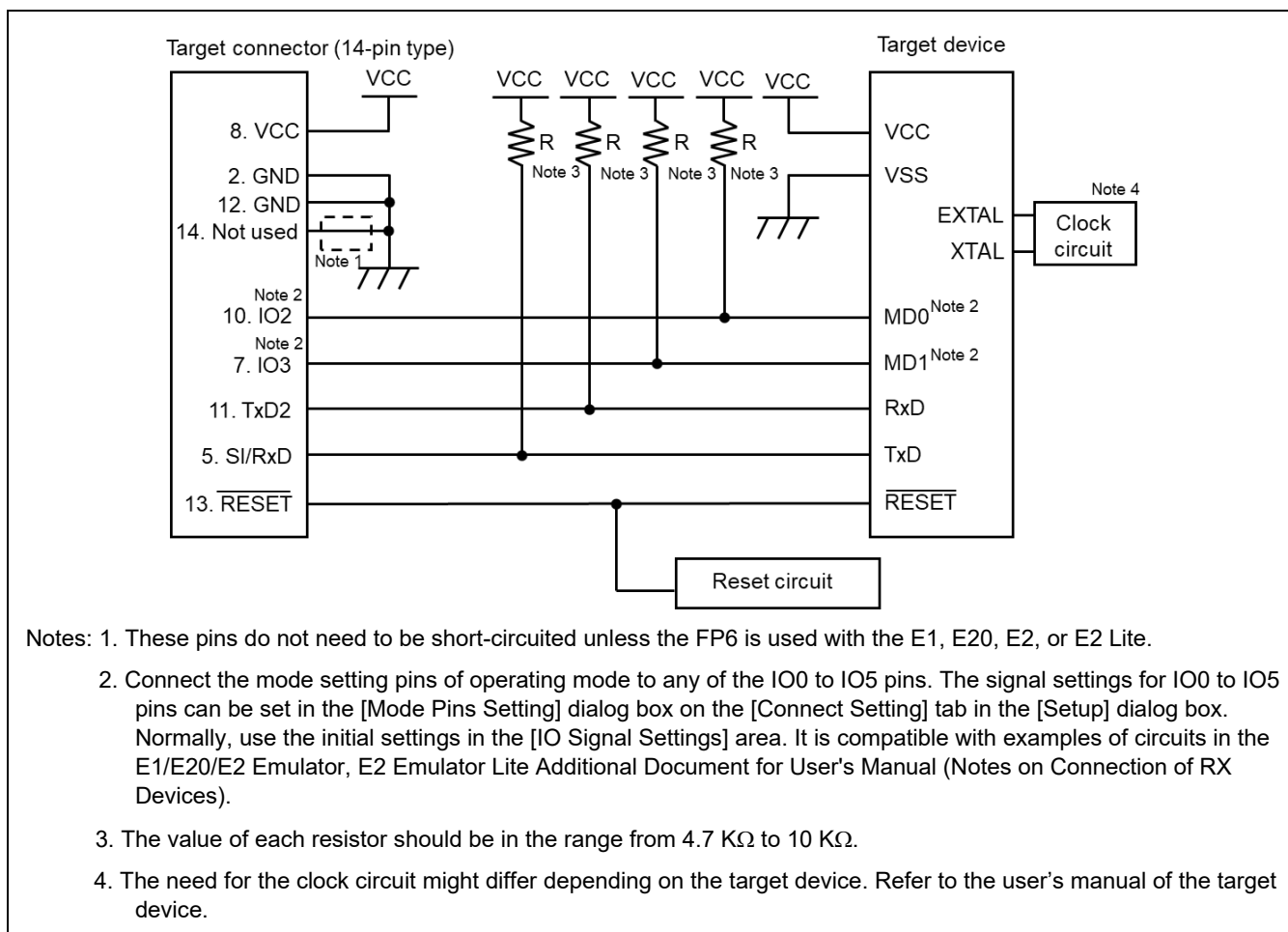
Figure 3.5 Example of a Circuit for RX Family and SuperH Family (SCI) (Case of RX62T)
