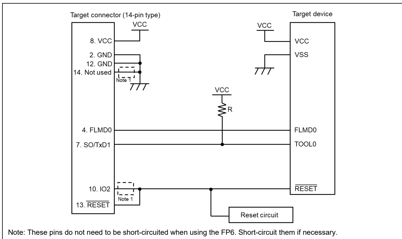
Figure 3.17 Example of a Circuit for 78K0R (Single-wire UART)
