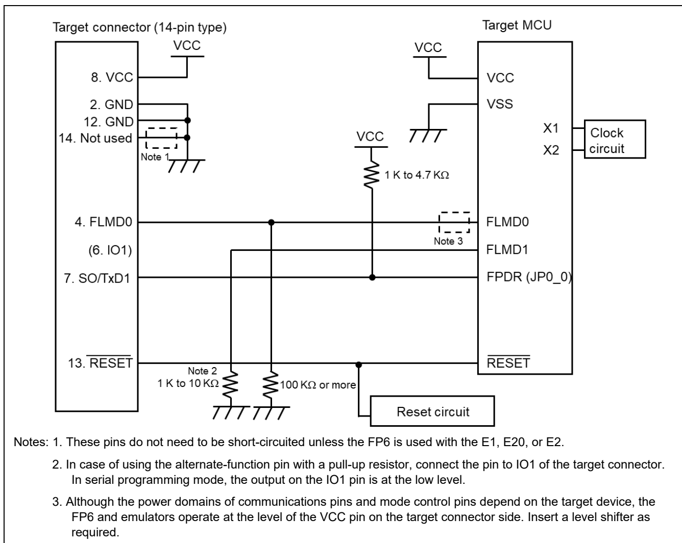
Figure 3.8 Example of a Circuit for RH850 Family (1-wire UART) (Case of RH850/F1x)
